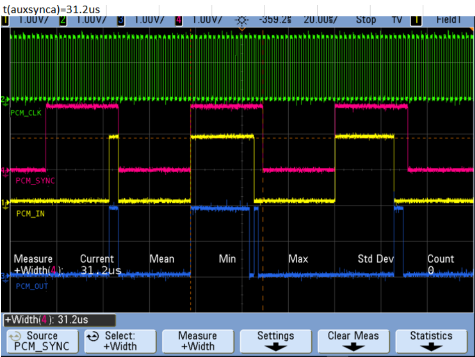
Figure 4-8: t(synch)
