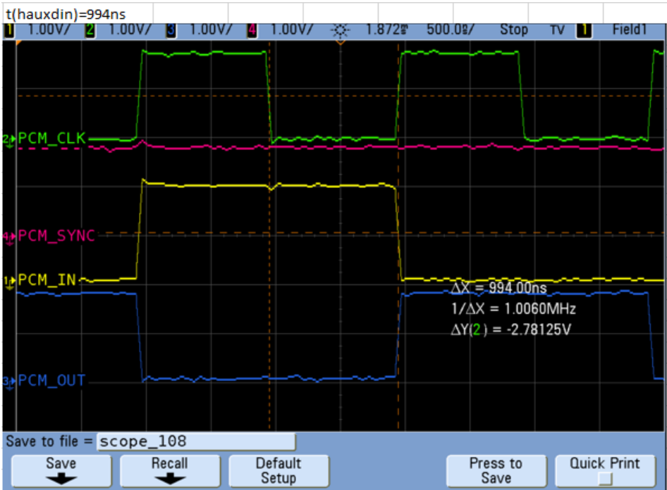
Figure 4-14: t(\text{hdin})
