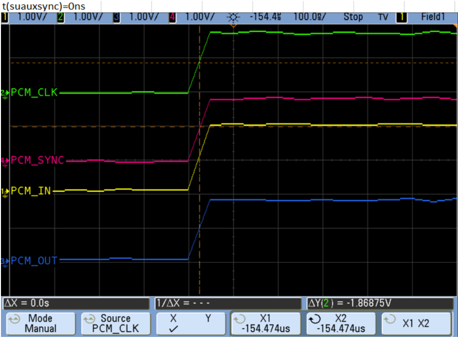
Figure 4-23: t(susync)
