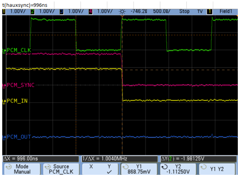
Figure 4-13: t(\text{hauxsync})
