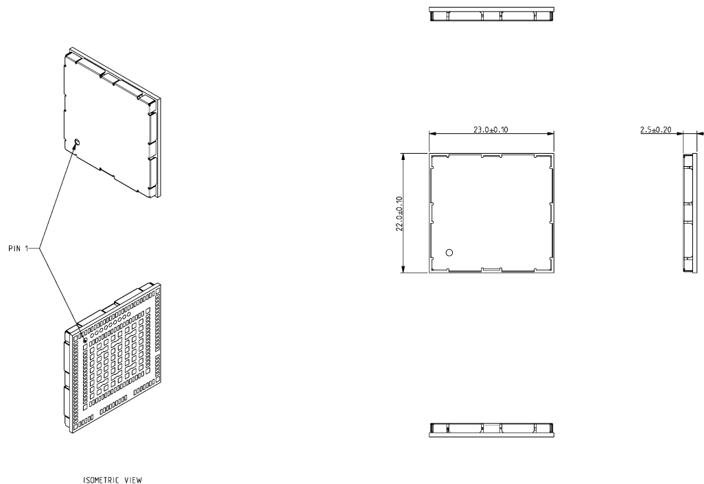
Figure 3-8: Mechanical Drawing 1
