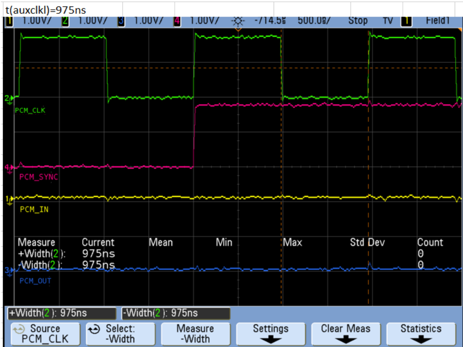
Figure 4-19: t(clkl)
