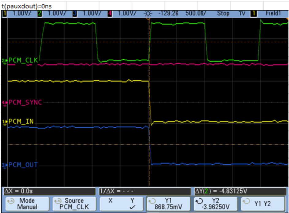
Figure 4-22: t(pauxdout)R
