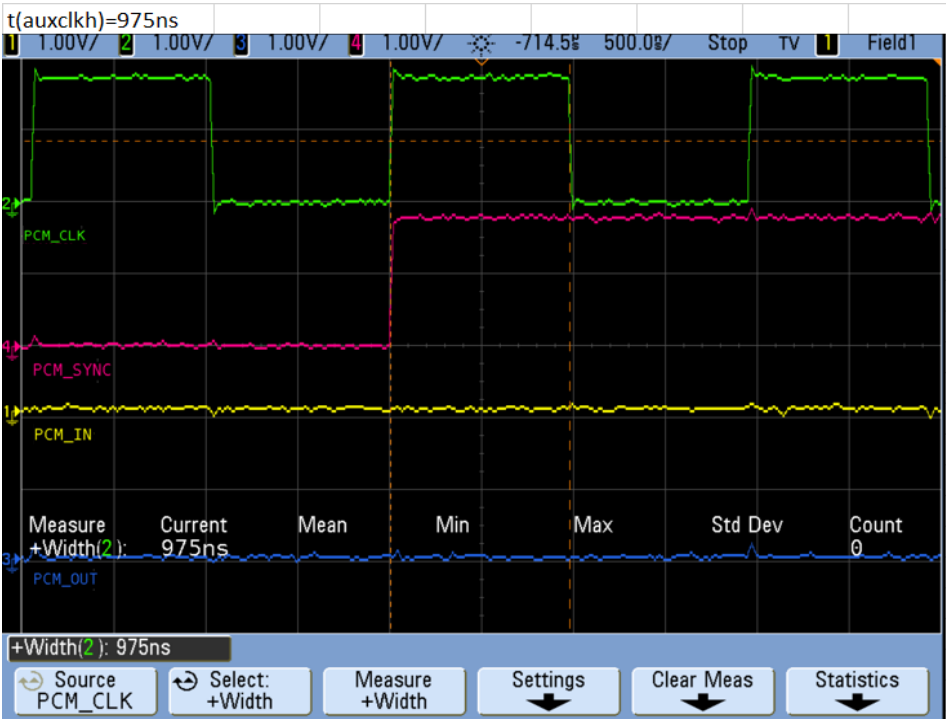
Figure 4-18: t(clkh)
