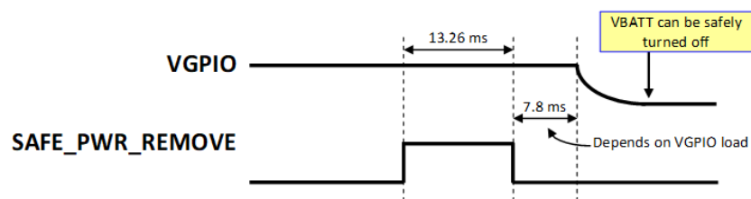
Figure 4-31: SAFE_PWR_REMOVE
