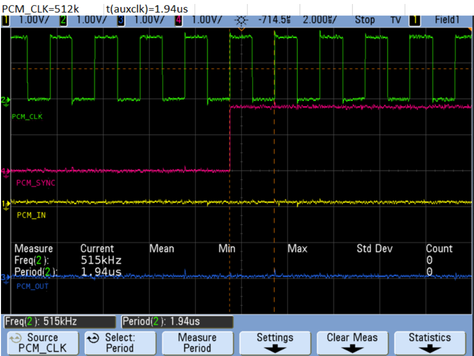
Figure 4-10: t(clk)
