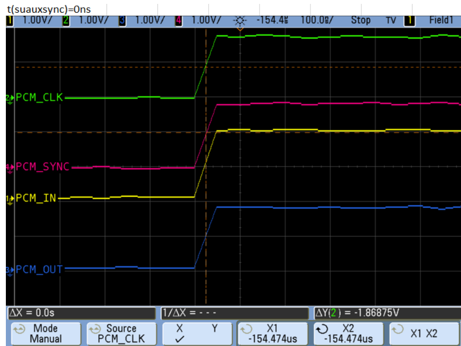
Figure 4-16: t(susync)
