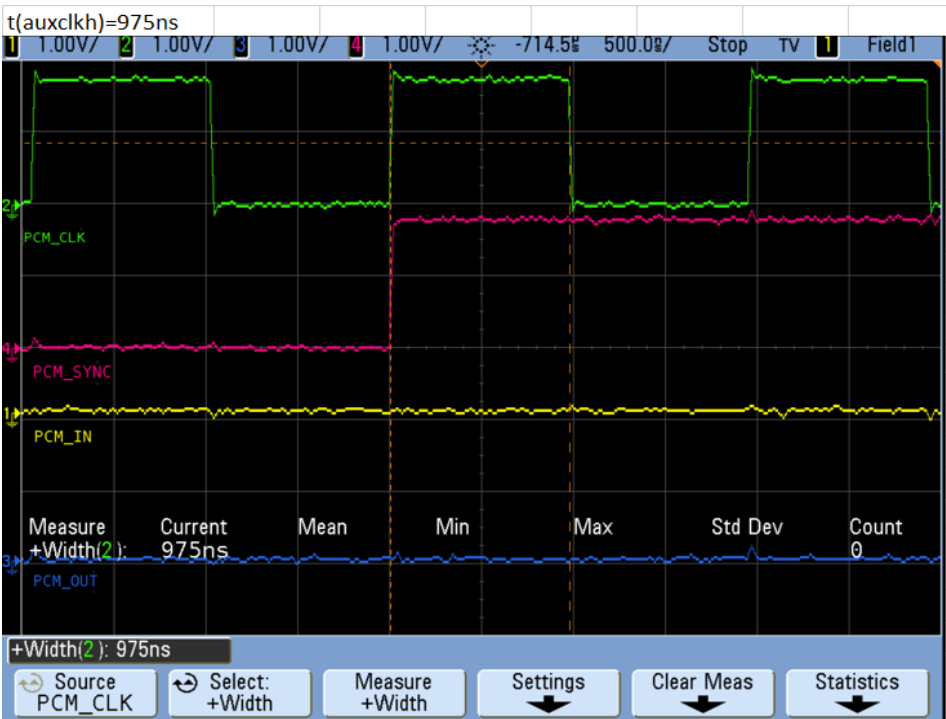
Figure 4-11: t(clkh)
