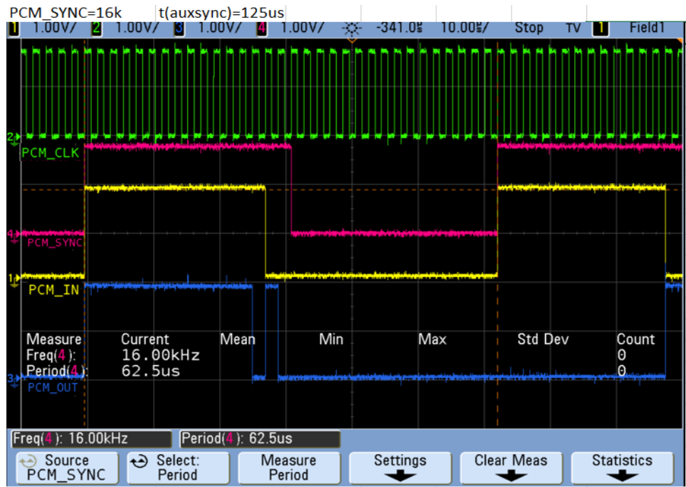
Figure 4-7: t(sync)
